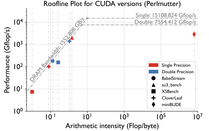
Fig. 1. Roofline plot for the most time-consuming kernel in the CUDA versions of each application, run on Perlmutter (NVIDIA A100). Red points are single precision, and blue points are double precision.
