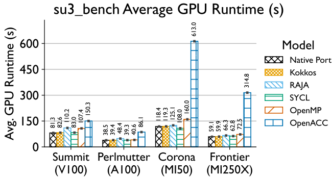
Fig. 3. Average GPU kernel execution time of the su3_bench proxy application across all platforms and programming models. Lower is better.
