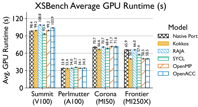
Fig. 2. Average GPU kernel execution time of the XSbench proxy application across all platforms and programming models. Lower is better.
