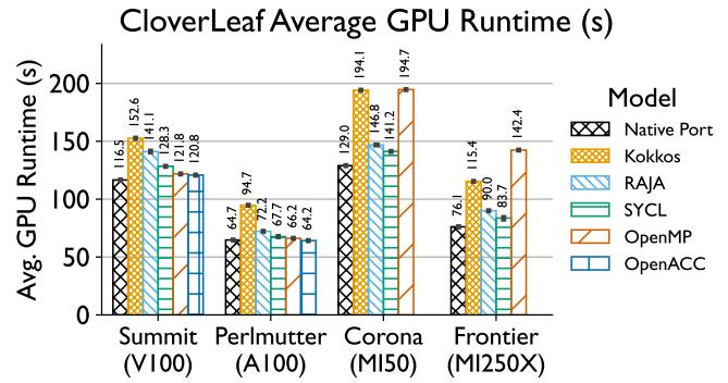
Fig. 4. Average GPU kernel execution time of the CloverLeaf proxy application across all platforms and programming models. Lower is better.
