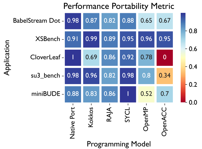
Fig. 7. \Phi of GPU kernel performance for each programming model and application combination. Applications are shown in ascending order of arithmetic intensity. Note for OpenACC we are unable to compile CloverLeaf on AMD systems.
