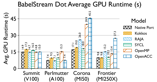
Fig. 5. Average GPU kernel execution time of the BabelStream Dot kernel across all platforms and programming models. Lower is better.
