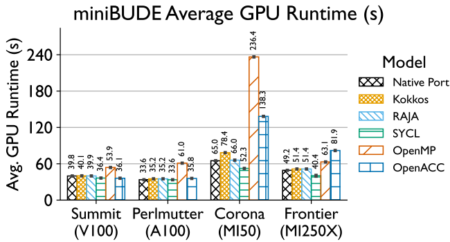
Fig. 6. Average GPU kernel execution time of the miniBUDE proxy application across all platforms and programming models. Lower is better.
